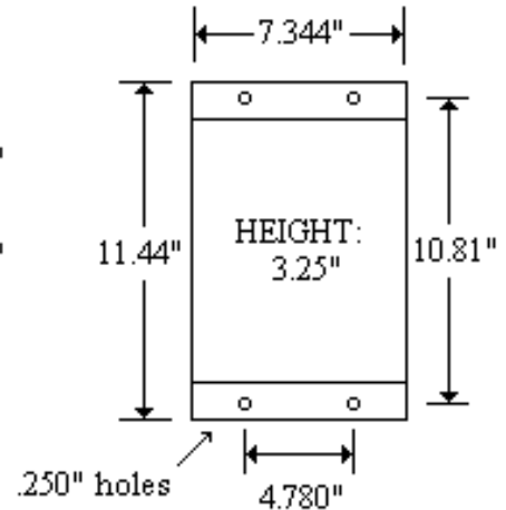
204/205 Series NEMA 1 enclosure
