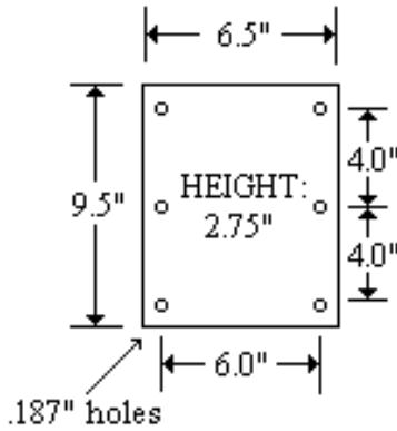
202 Series nylon standoffs
