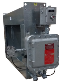
Figure 75. ULTRA-SAFE™ Explosion-proof Duct Heater
