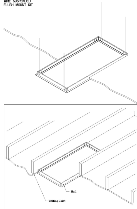
WIRE SUSPENDED FLUSH MOUNT KIT
