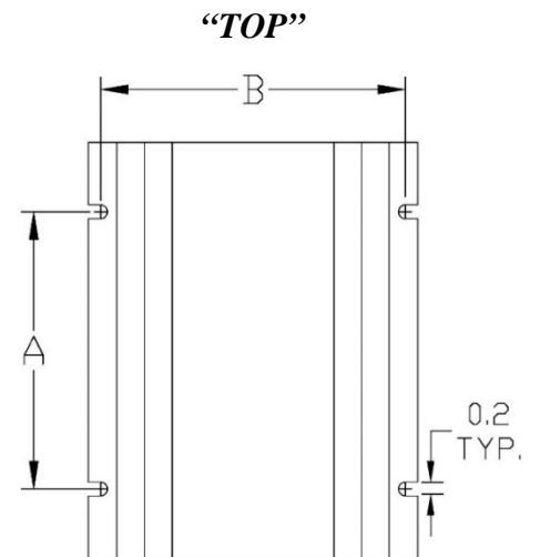
Mounting Dimensions
