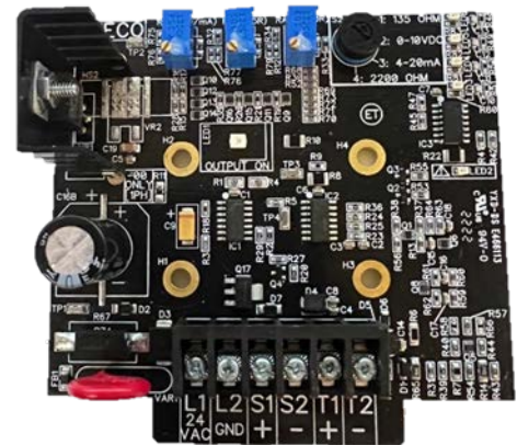
1 Model A Unit can drive up to 4 Model B controllers with 24VDC (Pulsed), 1 second time base.
