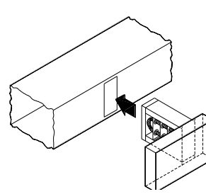
Fig. 2 - Installation drawing of slip-in heater.
