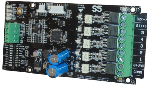
Figure 37. S5 Electronic Sequencer
