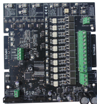
Figure 36. S10 Electronic Sequencers
