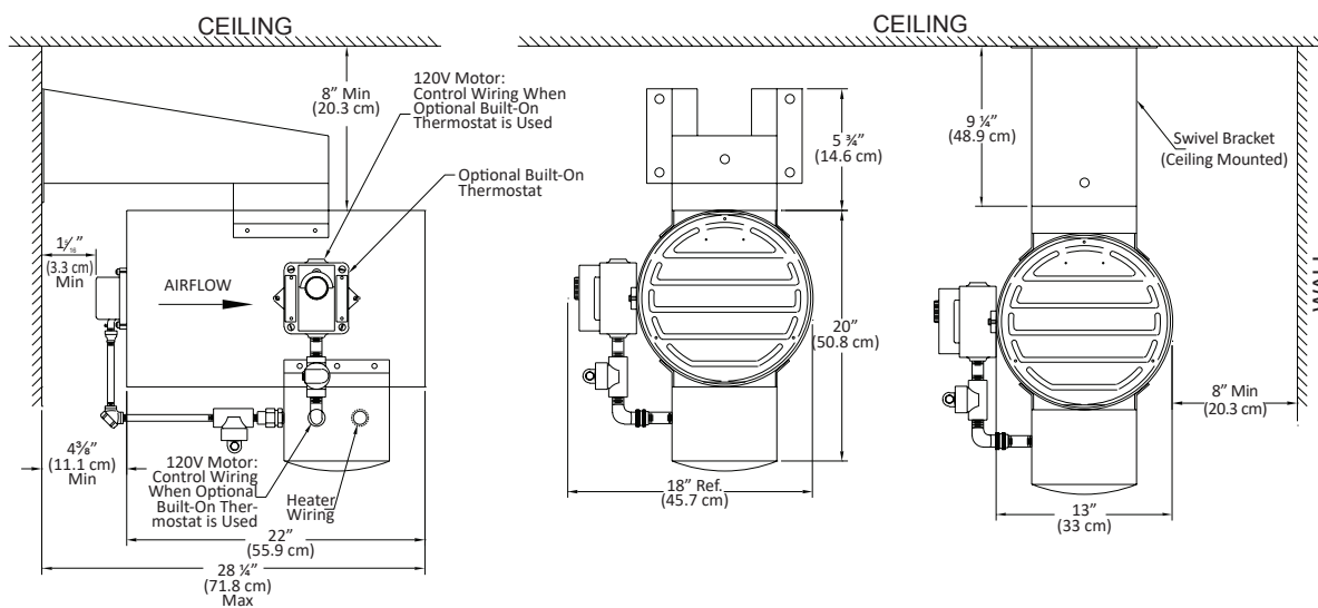
Standard Wall and Ceiling Installation with Swivel Mounting Bracket
