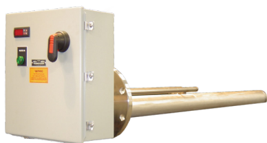
STORAGE TANK HEATING SYSTEMS
